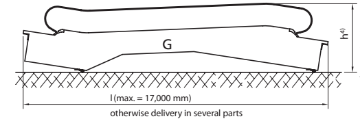
Transportation dimensions
